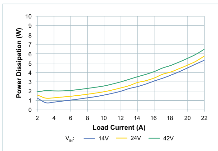
Figure 16 — System power dissipation, nominal trim, board temperature = -40^{\circ}\text{C}
