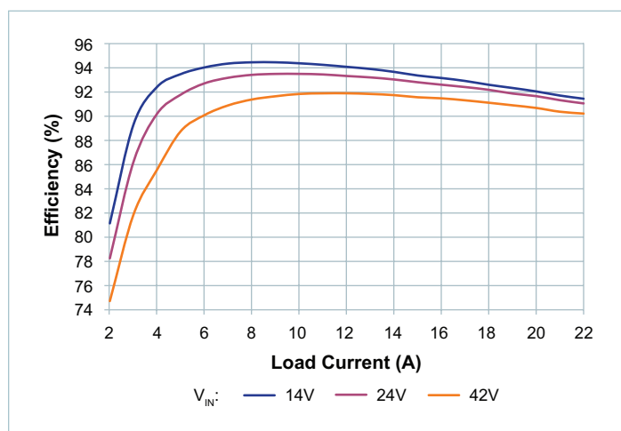
Figure 14 — System efficiency, low trim, board temperature = -40^{\circ}\text{C}
