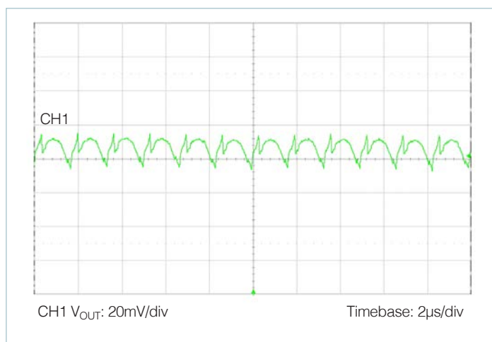
Figure 51 — Output voltage ripple: nominal line, nominal trim, 50% load, C_{OUT} = 12 \times 47\mu\text{F} ceramic
