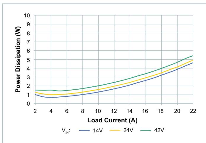
Figure 17 — System power dissipation, low trim, board temperature = -40^{\circ}\text{C}
