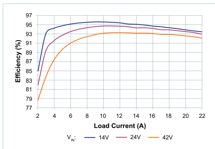
Figure 13 — System efficiency, nominal trim, board temperature = -40^{\circ}\text{C}
