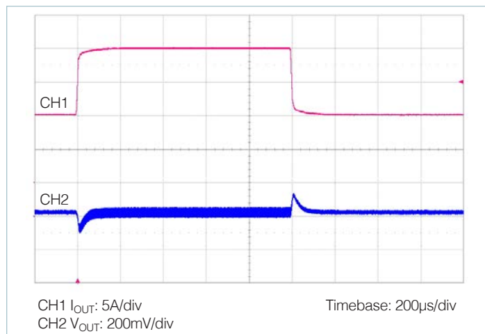
Figure 47 — Transient response: 50 – 100% load, at 1A/µs. nominal line, nominal trim, C_{OUT} = 12 \times 47\mu\text{F} ceramic
