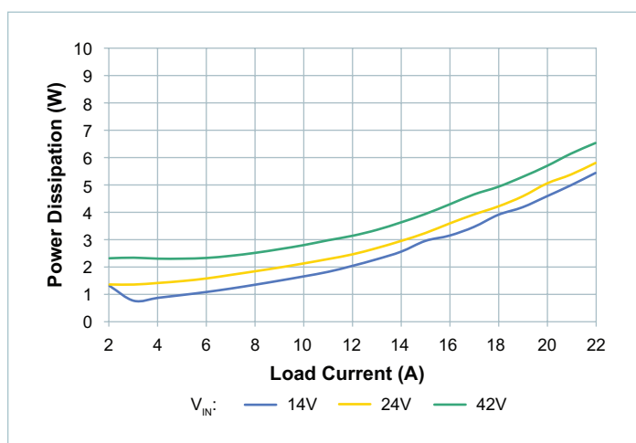
Figure 18 — System power dissipation, high trim, board temperature = -40^{\circ}\text{C}
