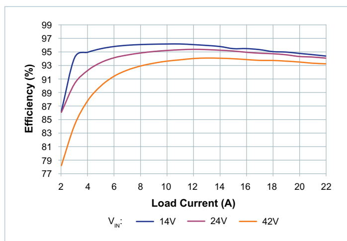
Figure 15 — System efficiency, high trim, board temperature = -40^{\circ}\text{C}
