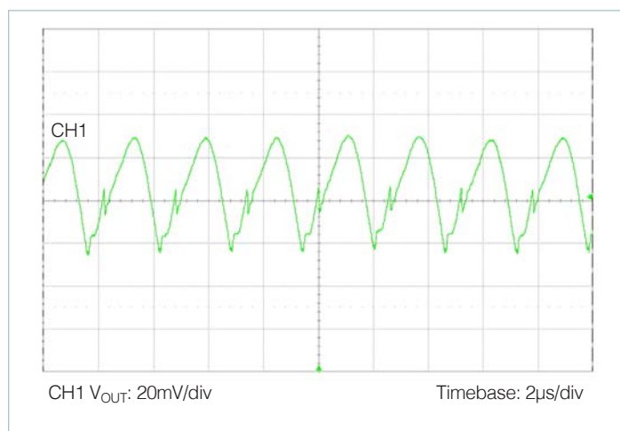
Figure 48 — Output voltage ripple: nominal line, nominal trim, 100% load, C_{OUT} = 12 \times 47\mu\text{F} ceramic
