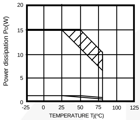
Figure 9. Power Dissipation vs. Temperature ( T_j )
