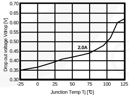
Figure 17. Dropout Voltage vs. Junction Temperature
