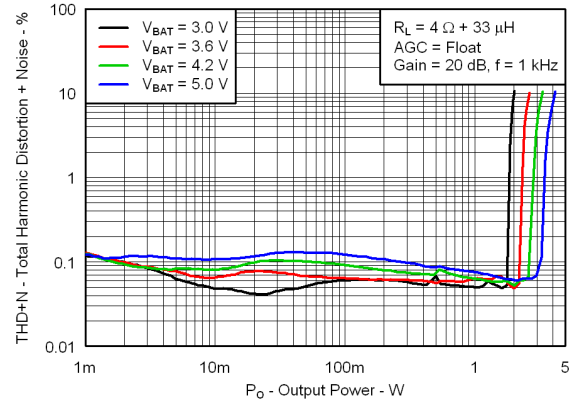
Figure 8. Total Harmonic Distortion + Noise vs Output Power
