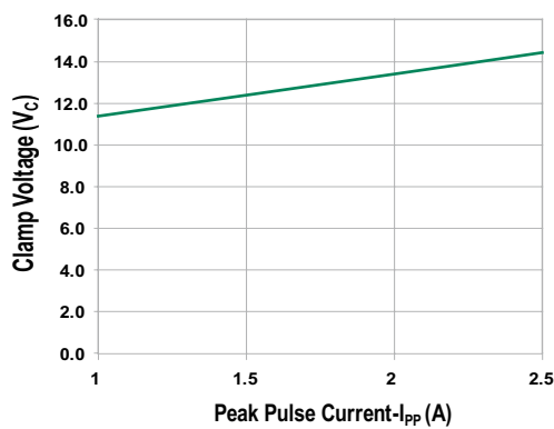
Clamping Voltage vs IPP
