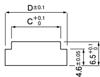
When mating with a standard type
