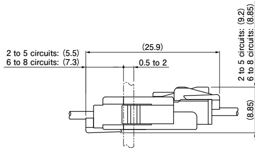
When mating with a retainer compatible type
