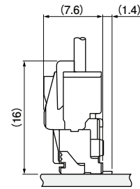
When mating with a retainer compatible type
