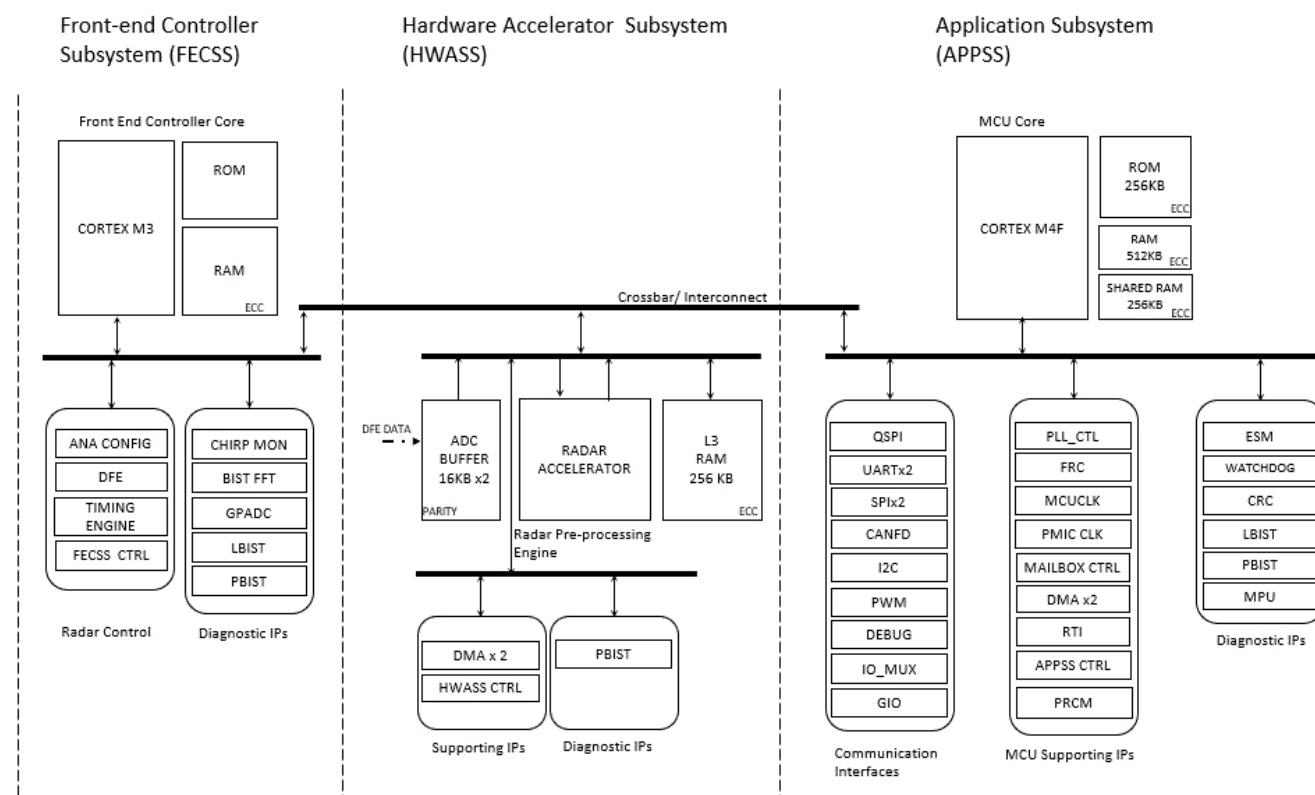
Figure 8-4. Processor Subsystem
