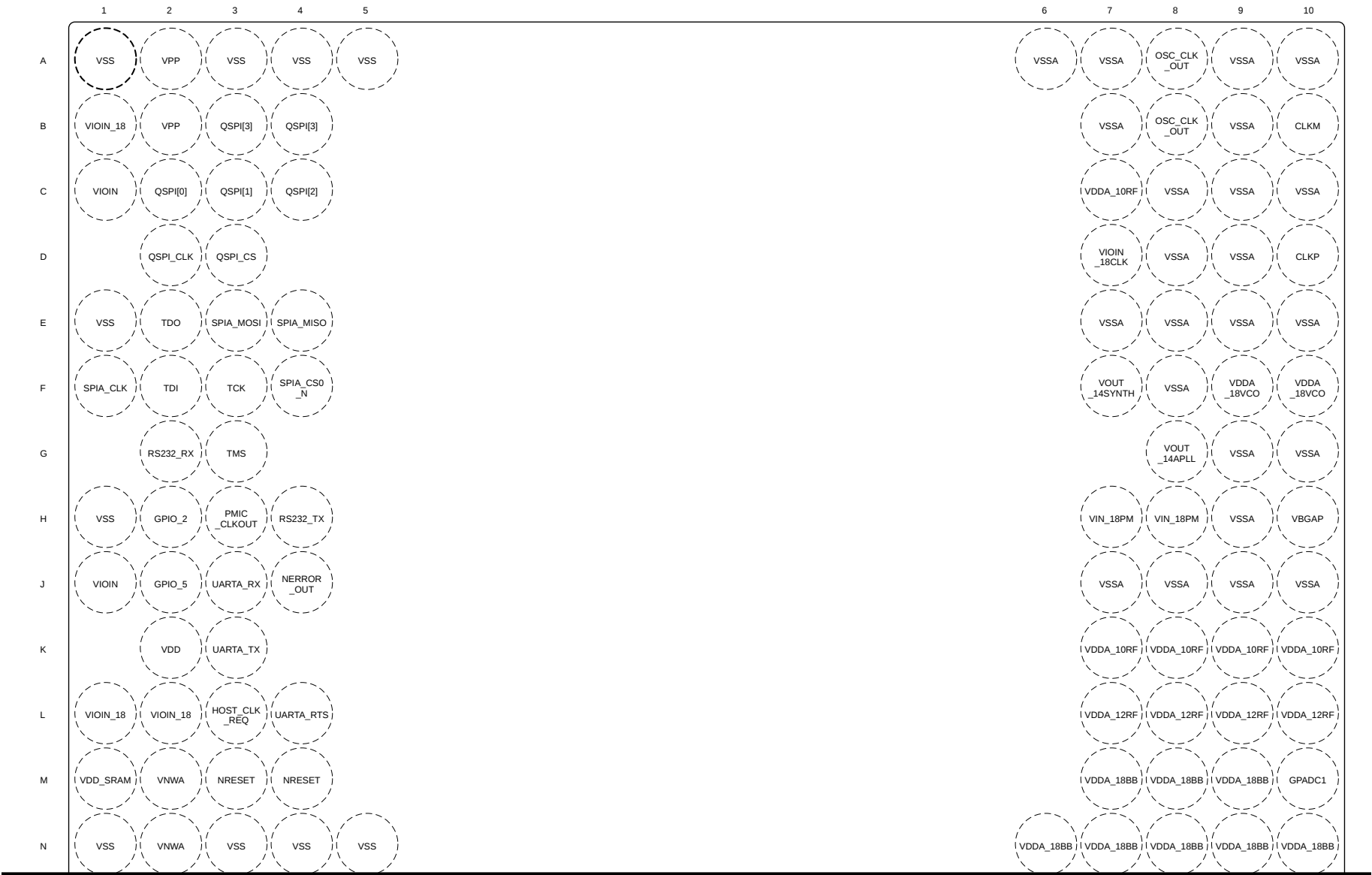
Figure 6-1. Pin Diagram (Top View)
