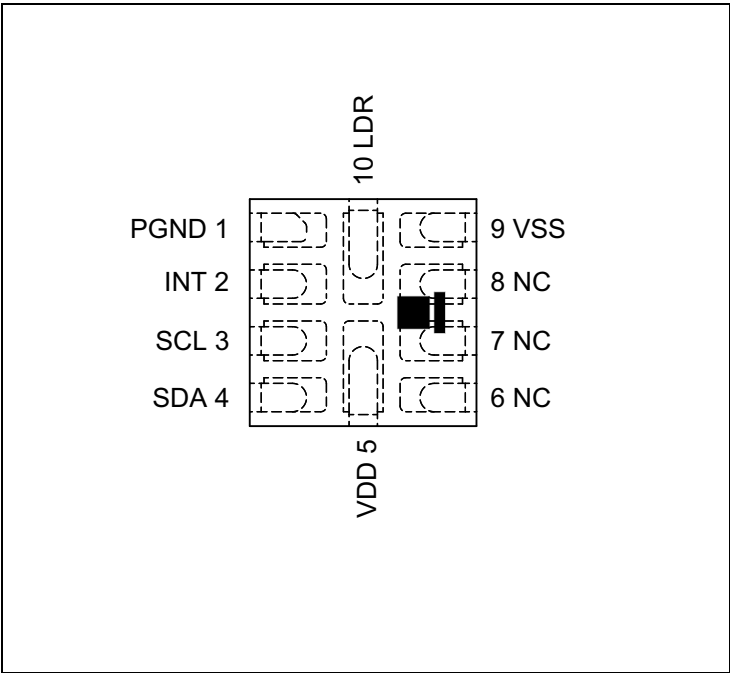
Figure 3: Pin Diagram of TSL2740
