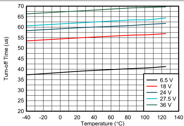
Figure 6-10. Turn-off Time ( t_{OFF} ) vs Temperature vs VS Voltage
