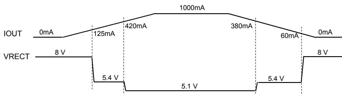
Figure A-8. VRECT changes by the value of output current. (Values shown are for reference.)
