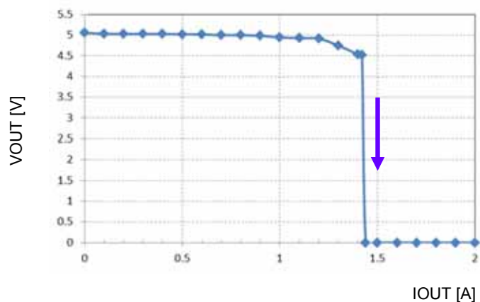
Figure B-7 VOUT vs IOUT
