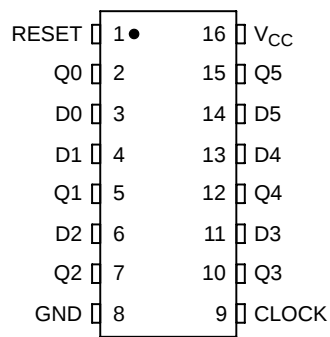
Figure 1. Pin Assignment
