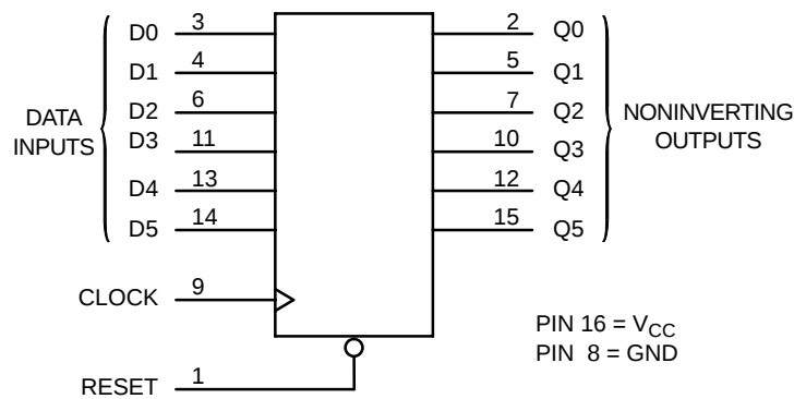
Figure 2. Logic Diagram
