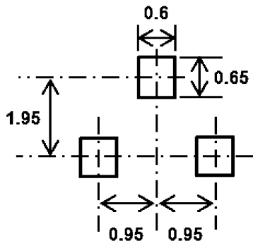
SOT23 (Unit: mm)
