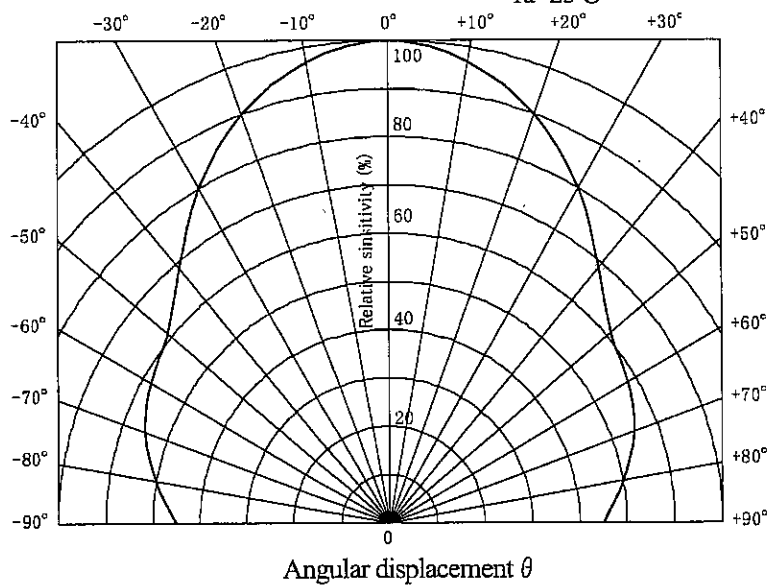
(3.5) Radiation diagram (For reference)
