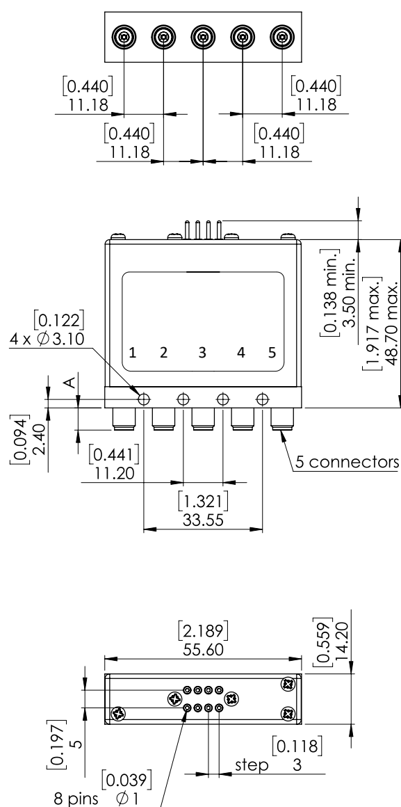
With solder pins
