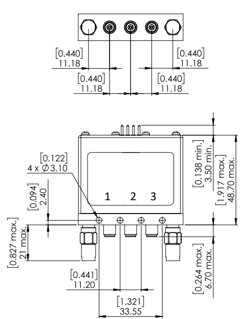
Model SMA2.9 with solder pins
