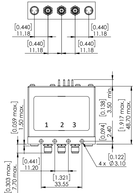
Model SMA2.9 with solder pins
