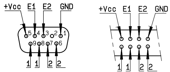
D-Sub connector
