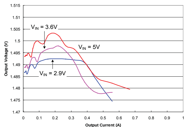
Load Regulation: MODE = Low
