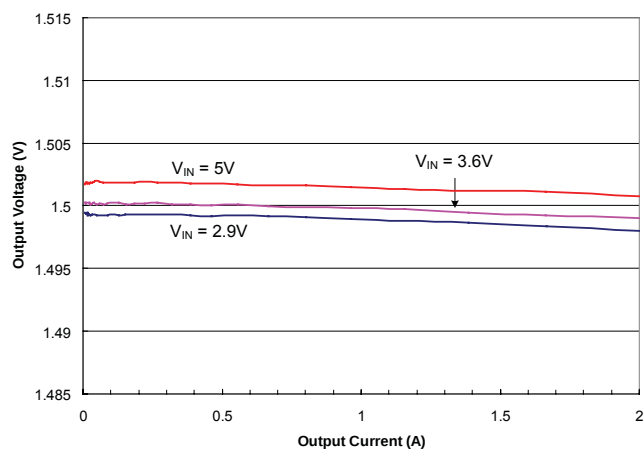
Load Regulation: MODE = High
