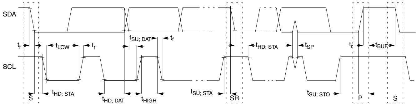
Figure 22. Timing definition for fast and standard mode devices on the I²C bus
