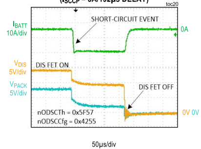
SHORT-CIRCUIT PROTECTION (I scpp = 5A/192μs DELAY)
