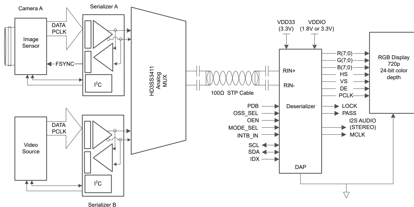
Figure 7-1. FPD Link III Application
