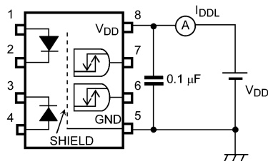
Fig. 12.1.3 IDDL Test Circuit
