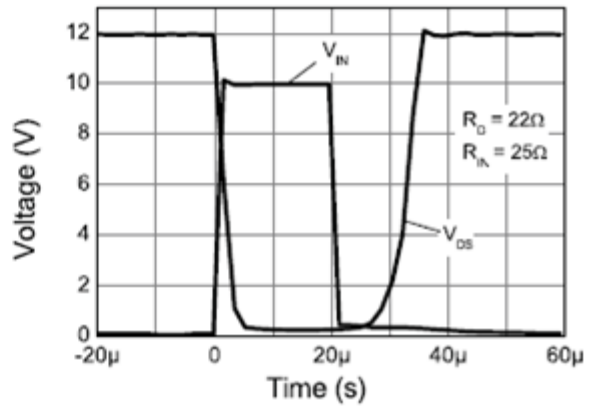
Switching Speed
