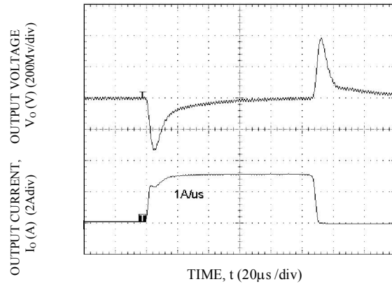
Transient Response to Dynamic Load Change from 0% 50% to 0%. V_o=1.2V
