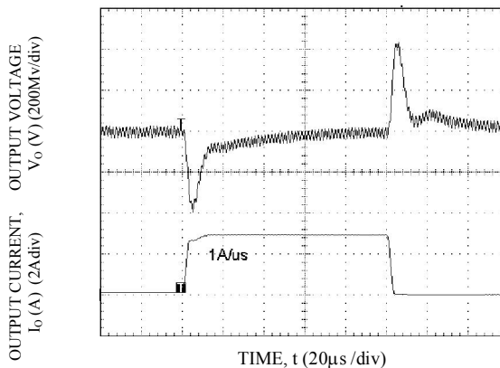
Transient Response to Dynamic Load Change from 0% 50% to 0%. V_o=3.3V
