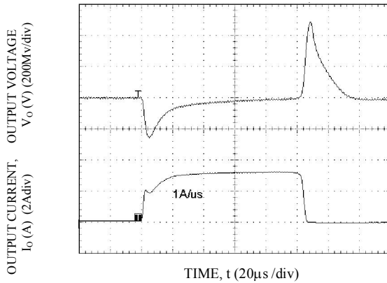
Transient Response to Dynamic Load Change from 0% 50% to 0%. V_o=0.6V
