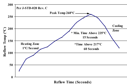
Recommended linear reflow profile using Sn/Ag/Cu solder.
