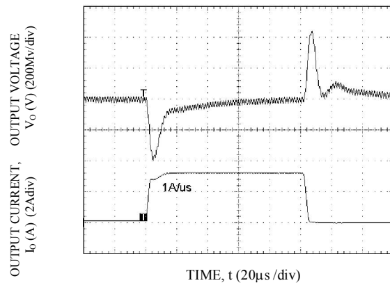
Transient Response to Dynamic Load Change from 0% 50% to 0%. V_o=2.5V
