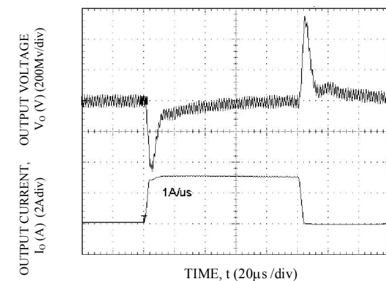
Transient Response to Dynamic Load Change from 0% 50% to 0%. V_o=5.0V
