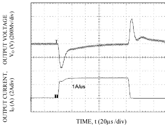
Transient Response to Dynamic Load Change from 0% 50% to 0%. V_o=1.8V
