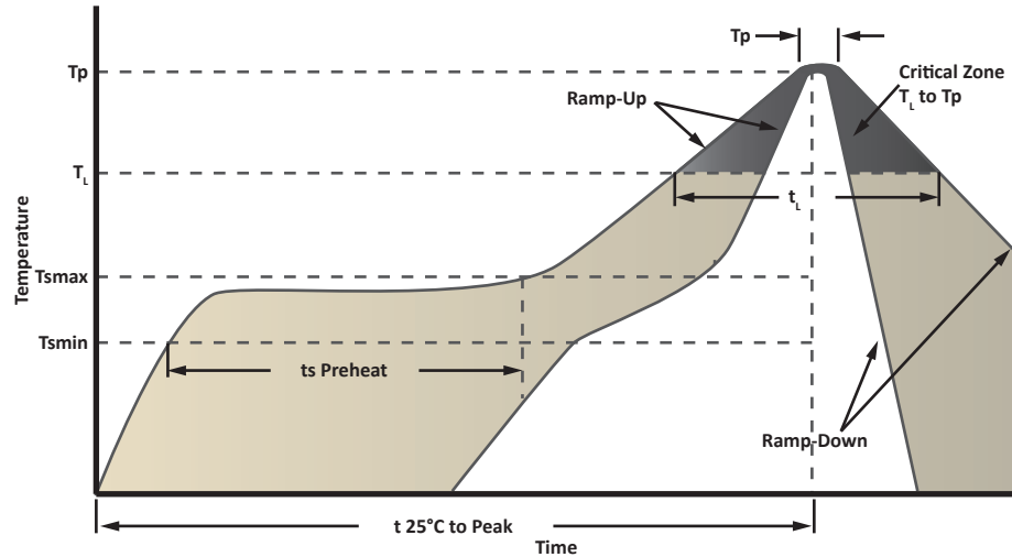
FIGURE 1 SOLDER WAVEFORM
