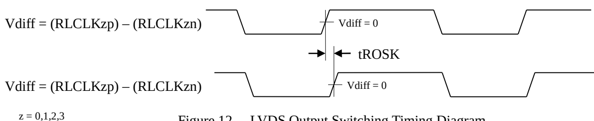
Figure 12. LVDS Output Switching Timing Diagram
