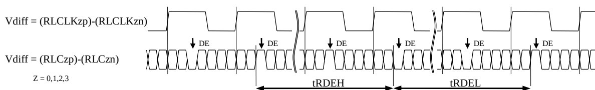
Figure 15. DE Period Requirement
