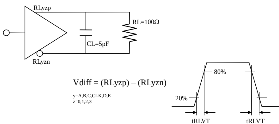
Figure 10. LVDS Output Switching Timing Diagram and Test Circuit
