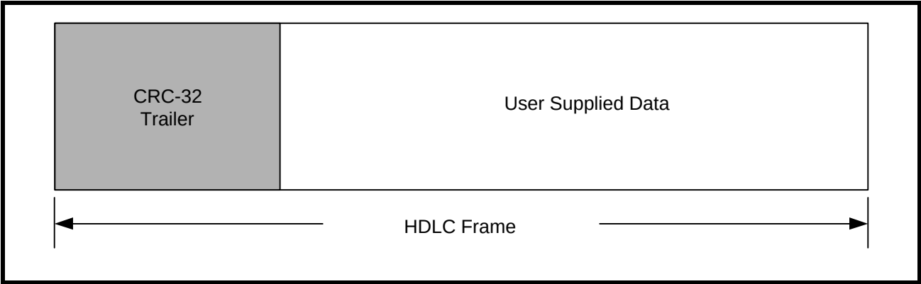
FIGURE 202. AN OUTBOUND HDLC FRAME WHEN CRC-32 IS SELECTED.
