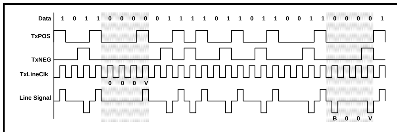
FIGURE 169. ILLUSTRATION OF TWO EXAMPLES OF HDB3 ENCODING
