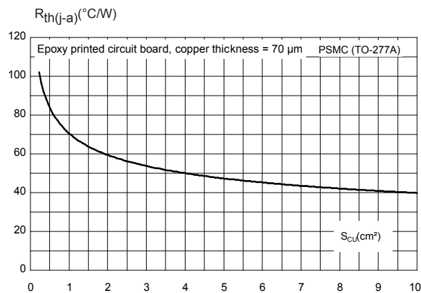
Figure 11. Thermal resistance junction to ambient versus copper surface under tab (typical values, epoxy printed board FR4, e_{Cu} = 70 μm) (PSMC (TO-277A))
