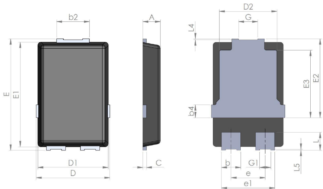
Figure 12. PSMC (TO-277A) package outline
