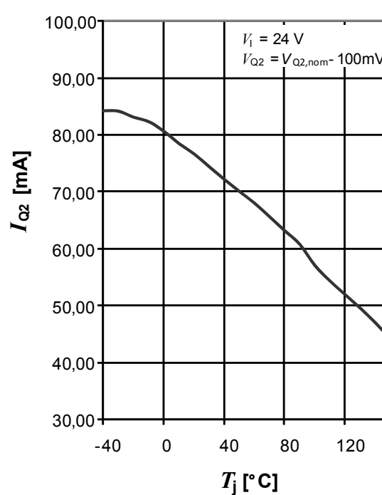
Output Current Limitation I_{Q2} versus Junction Temperature T_j (@ V_{Q2,nom} - 100\text{mV} )
