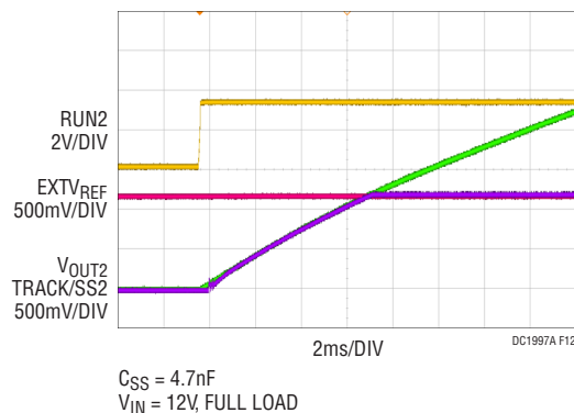
Figure 12. Turn-On of the 1.2V Rail of the DC1997A-B Assembly. RUN Pin Released from Ground
