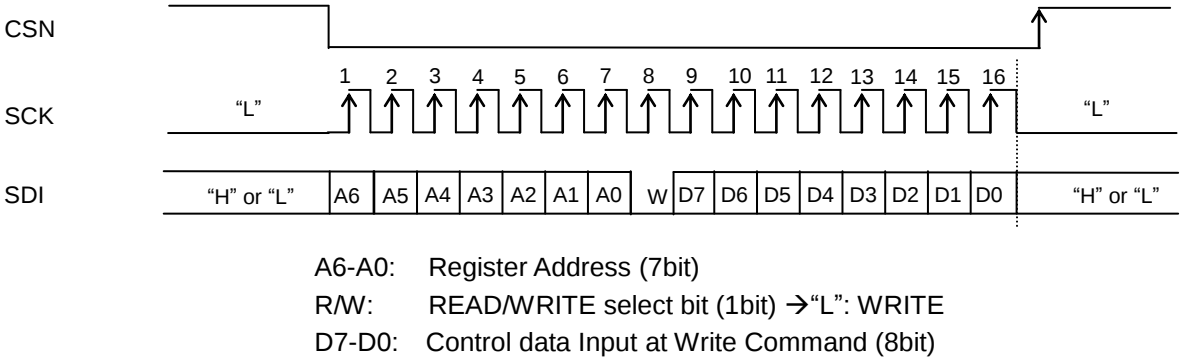
Figure 4. Serial Control Interface Timing (write mode)
