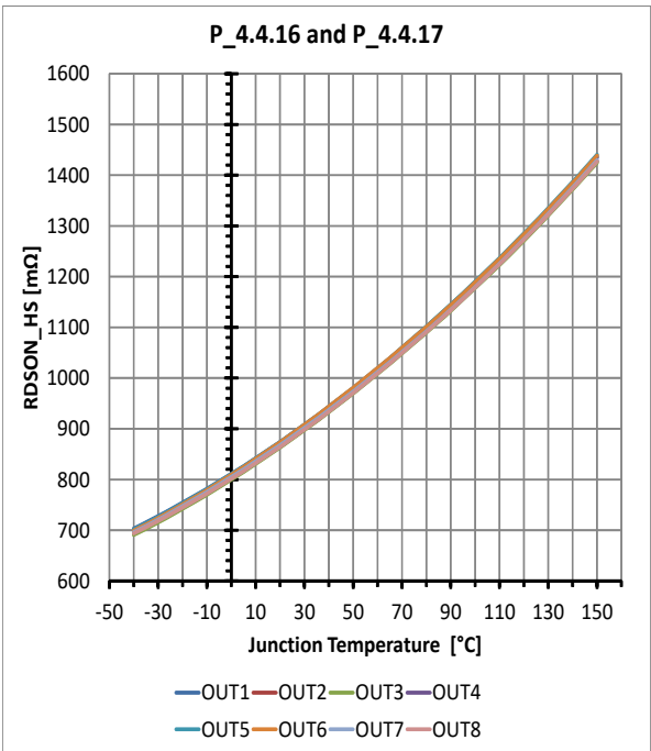
HS static drain-source ON-resistance VS = 13.5V and VDD = 5V
