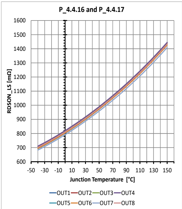
LS static drain-source ON-resistance VS = 13.5V and VDD = 5V
