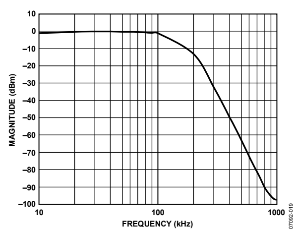
Figure 22. Receive GSM Baseband Filter Response
