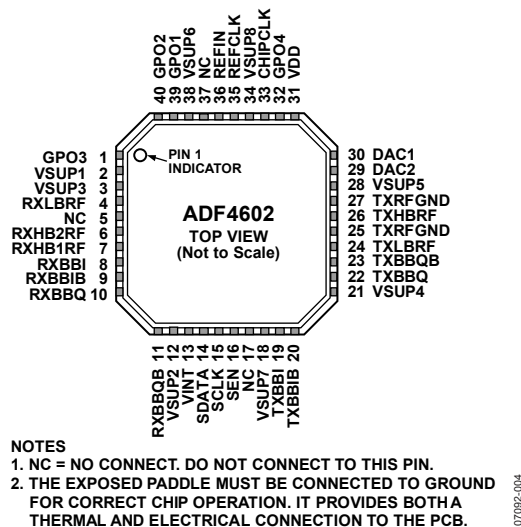
Figure 4. Pin Configuration
