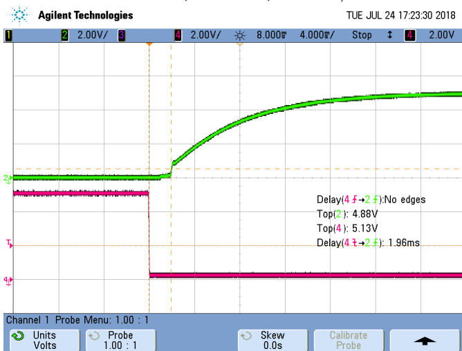
On/Off Enable Delay (Vin = 12V Vout= nom Iload =0A Load=330μF CH2: Vout; CH4: Enable; Ta=+25°C)
