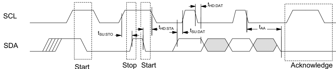
Figure 19. Write Bus Timing Diagram
