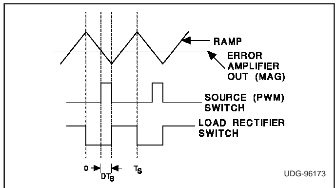
Figure 3. Circuit waveforms.
