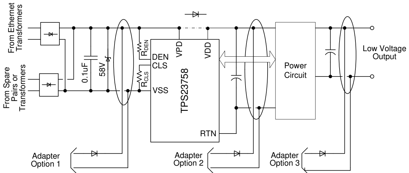
Figure 7-10. ORing Configurations
