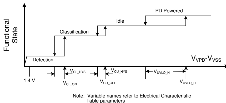
Figure 7-5. Threshold Voltages
