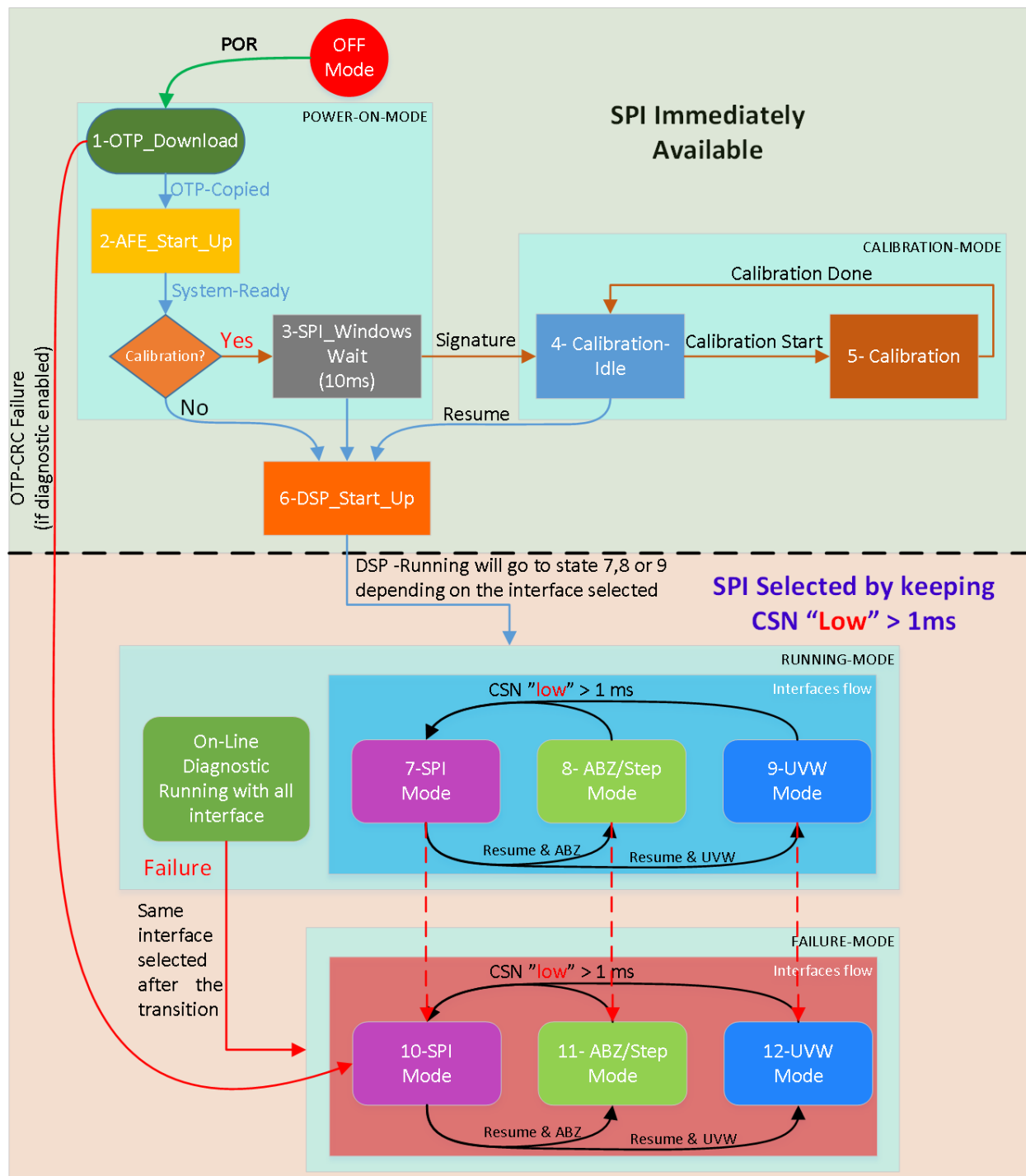
Figure 6: Operation modes and transitions
