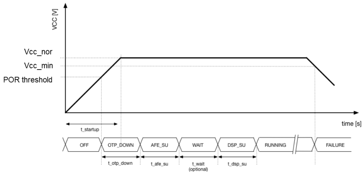
Figure 8: Normal operation with under voltage diagnostic
