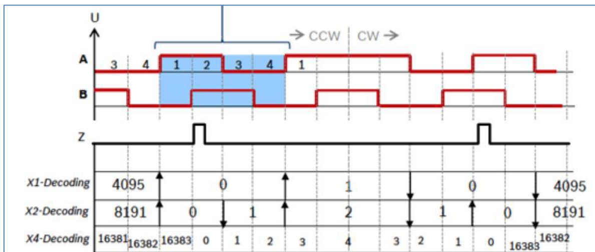
Figure 19: Behavior of Z-pulse
