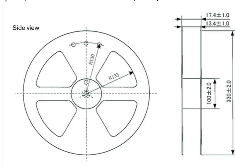
Figure 36: Specification of reel
