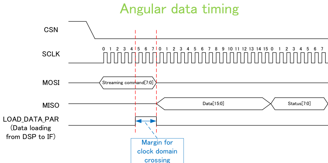
Figure 30: Angular data timing
