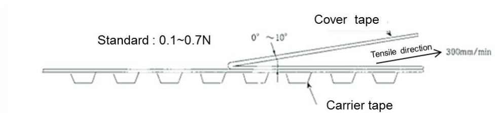
Figure 35: Peel strength
