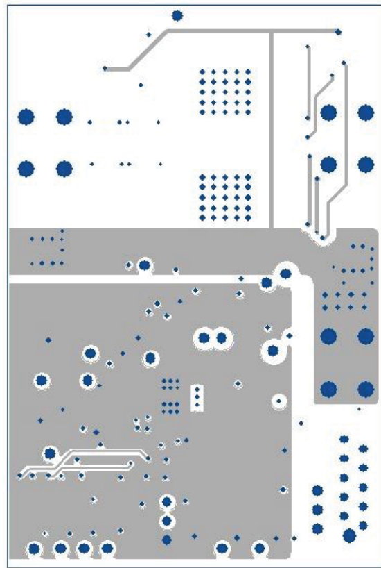
Figure 9. Inner Layer 3
