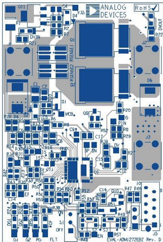
Figure 7. Top Layer 1
