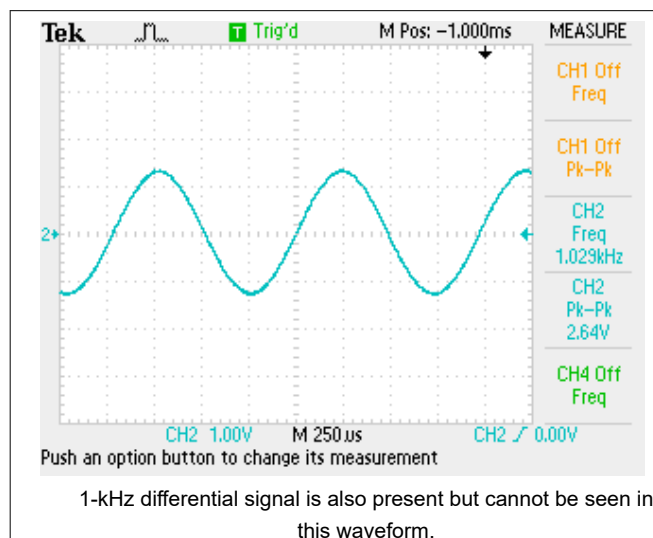
Figure 9-4. Input of Typical Application Showing 60-Hz Common-Mode Signal
