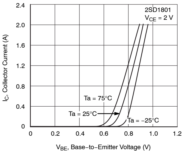
Figure 7. I_C - V_{BE}
