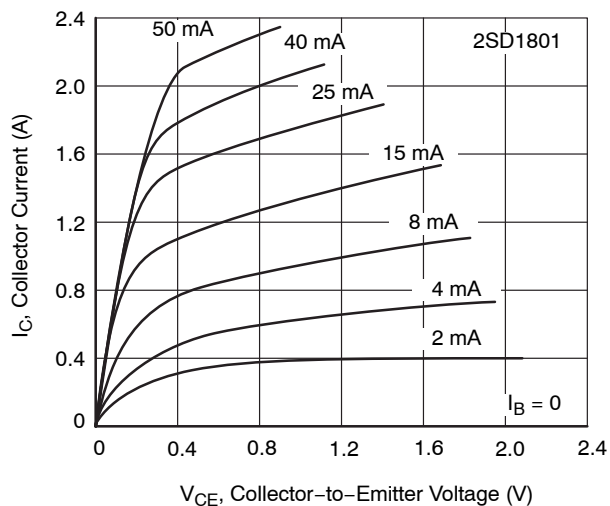
Figure 3. I_C - V_{CE}
