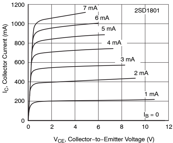
Figure 5. I_C - V_{CE}
