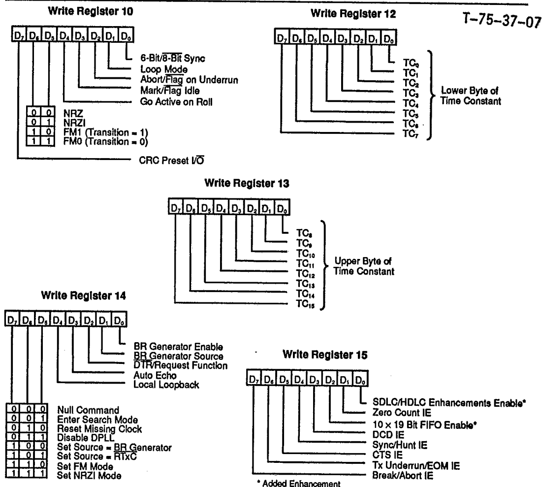
Figure 9. Write Register Bit Functions (continued)
