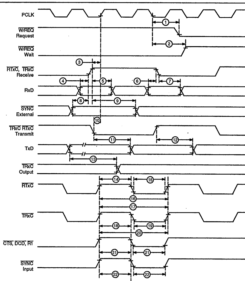
Figure 19. General Timing
