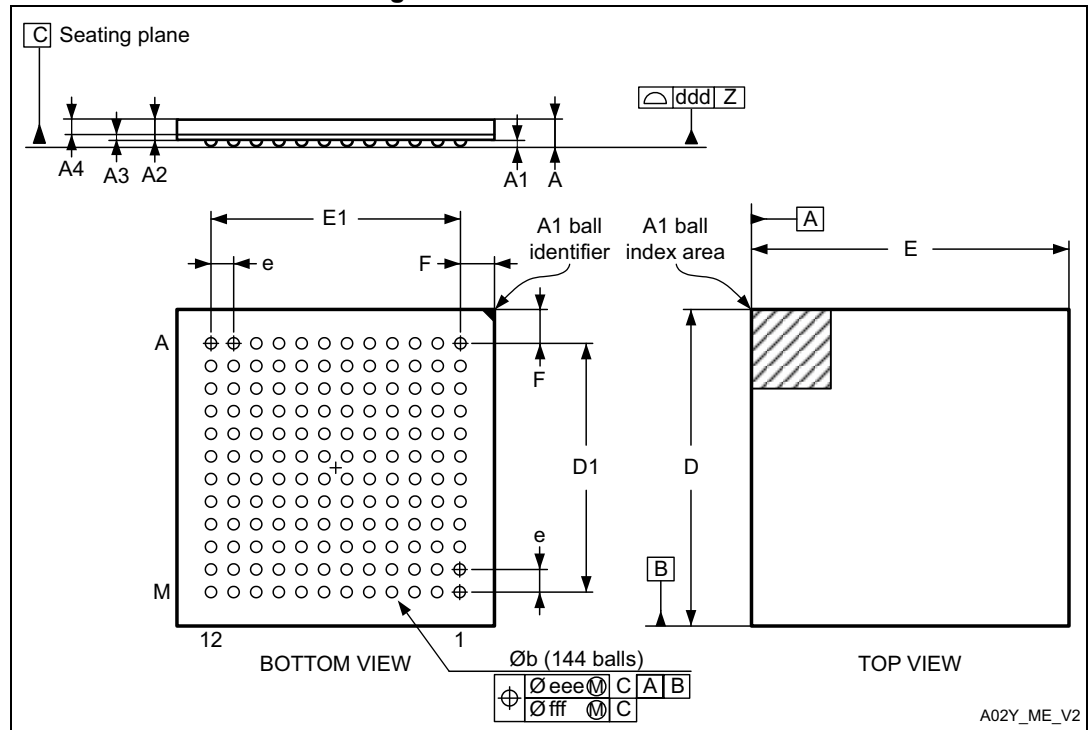
Figure 75. UFBGA144 outline
