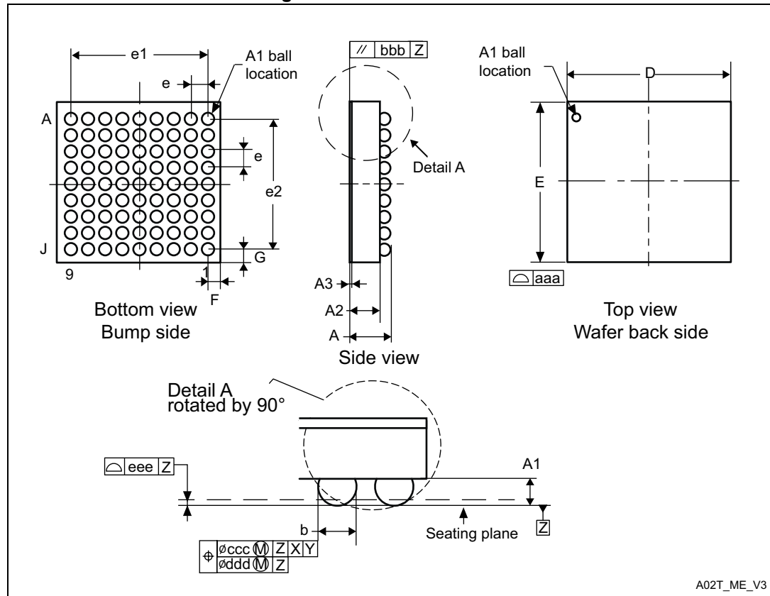
Figure 77. WLCSP81 outline
