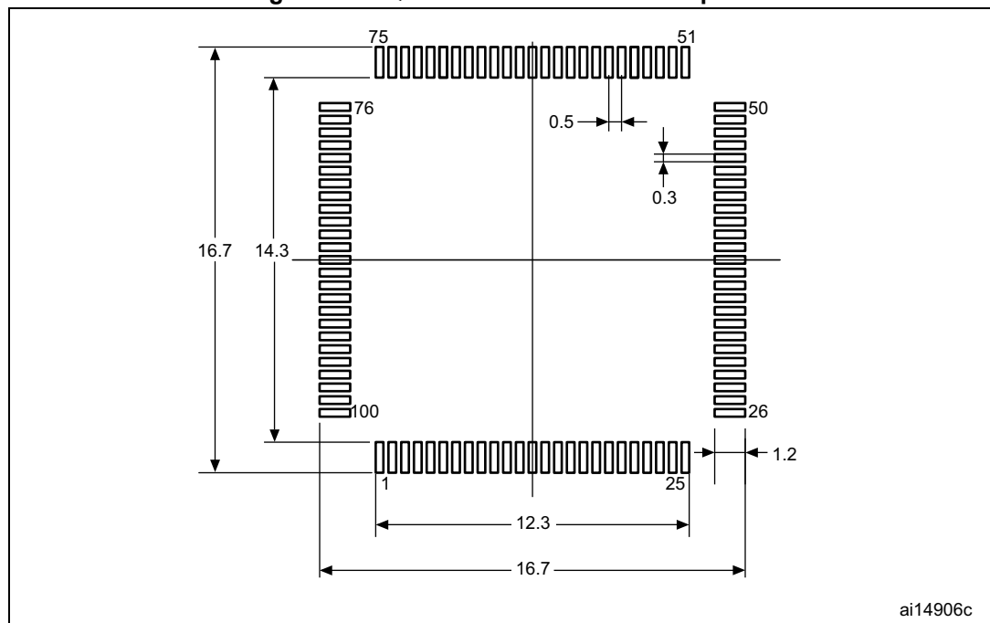
Figure 70. LQFP100 recommended footprint
