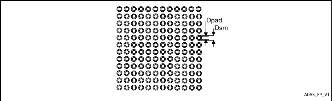
Figure 74. UFBGA144 recommended footprint
