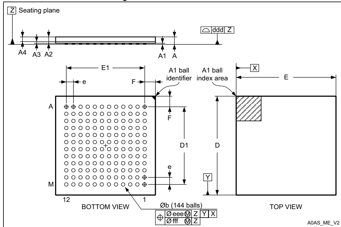
Figure 73. UFBGA144 outline
