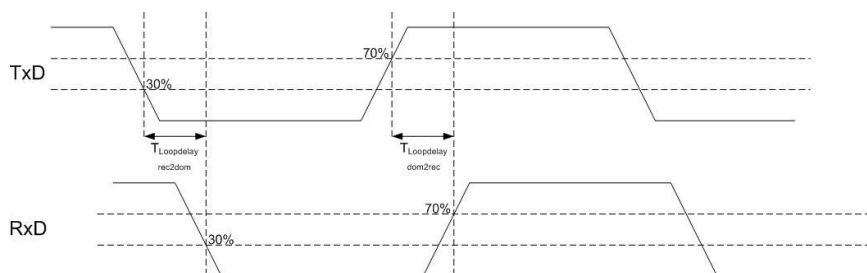
Figure 2: Transceiver Loop delay specification
