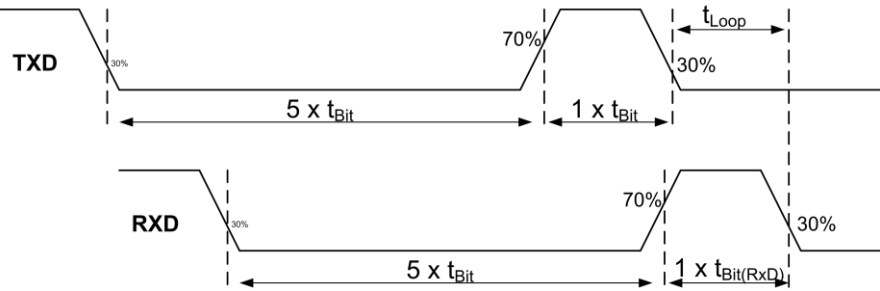
Figure 4: Transceiver Loop delay symmetry specification
