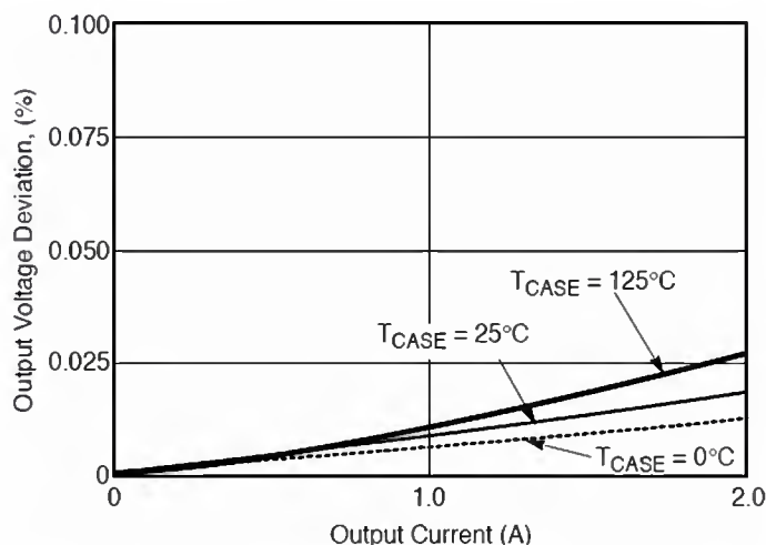
Figure 3. Load Regulation vs. Output Current
