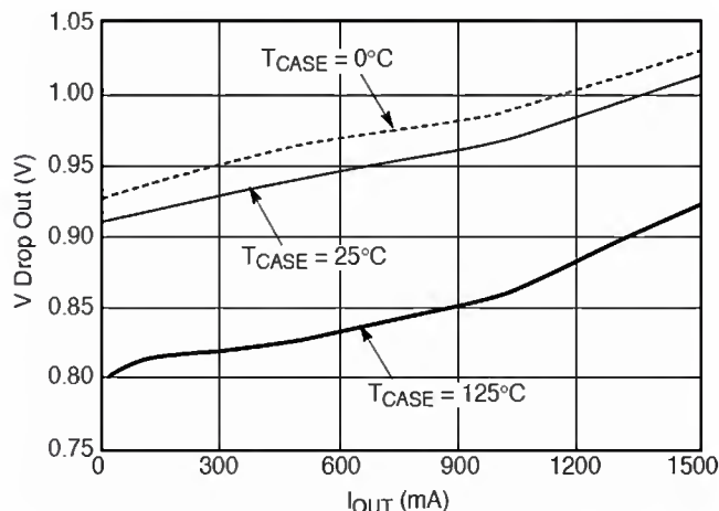
Figure 1. Vdrop vs. Output Current
