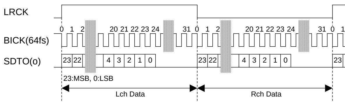
Figure 1. Mode 0 Timing
