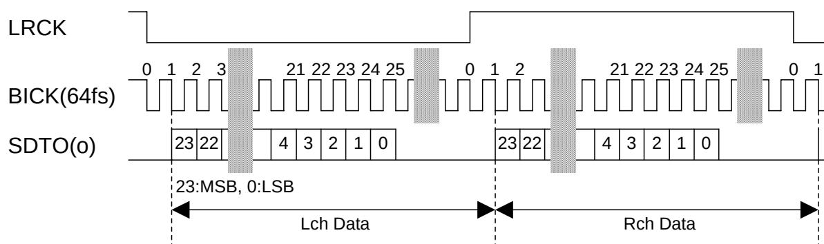
Figure 2. Mode 1 Timing
