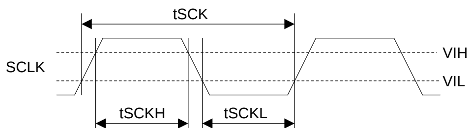
Clock Timing
