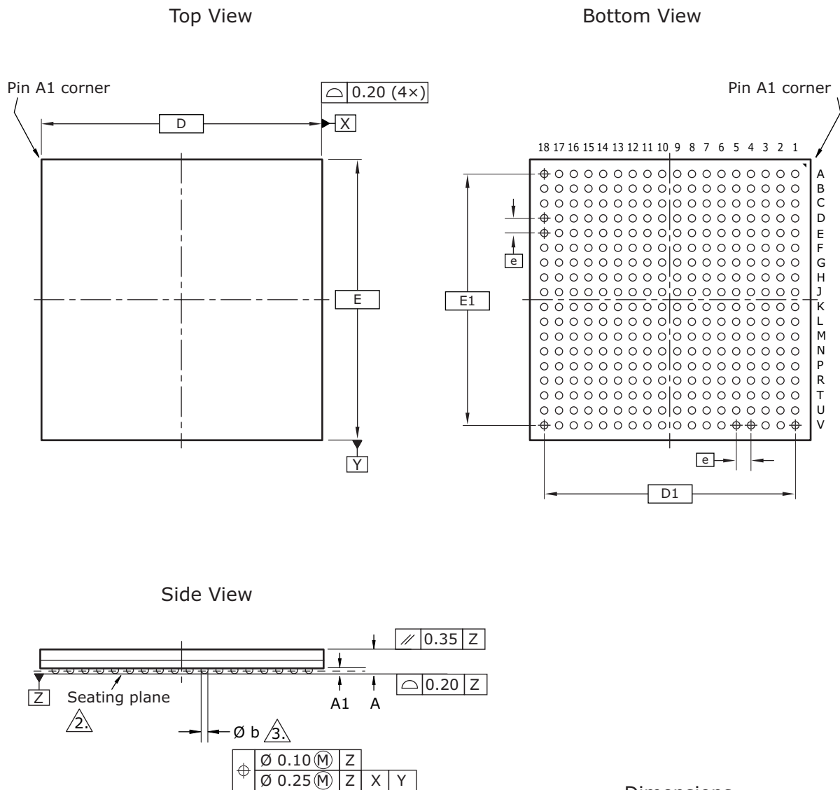
Figure 193 • Package Drawing
