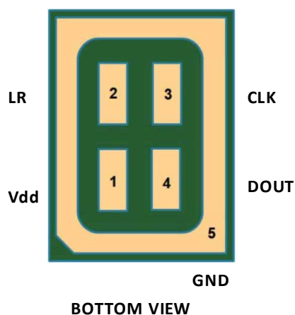
Figure 1. Pin connections
