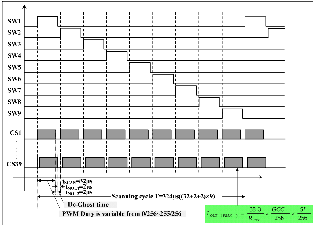
Figure 11 Scanning Timing
