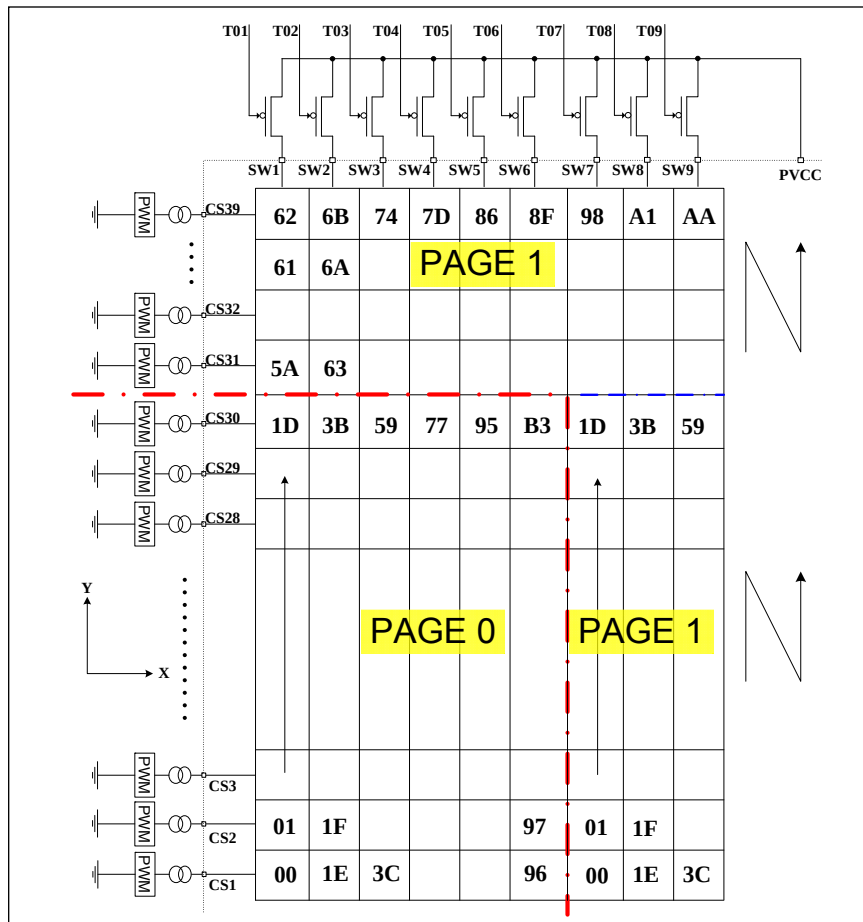
Figure 8 PWM Register
