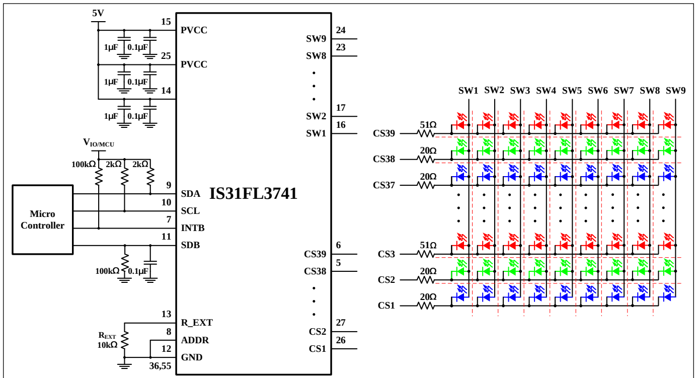
Figure 2 Typical Application Circuit (RGB Color: 13×9)
