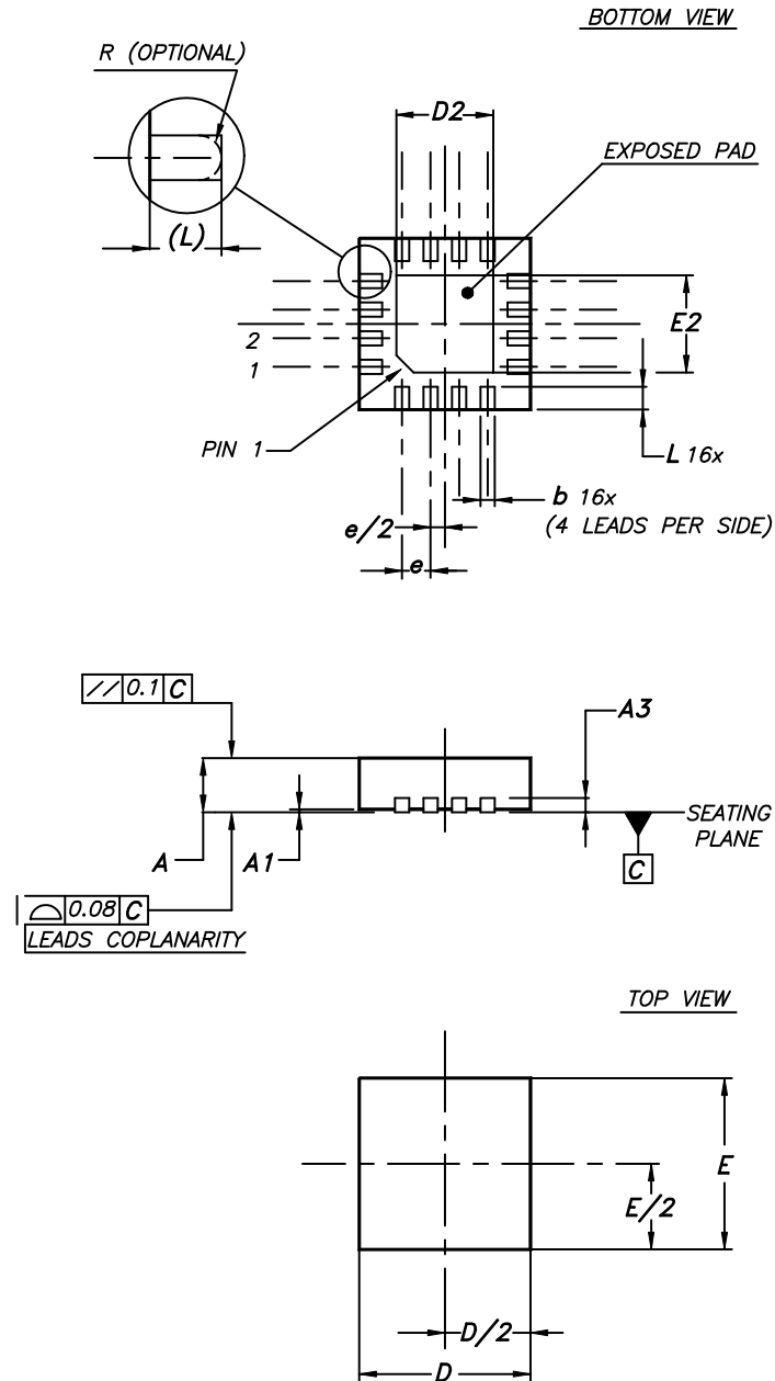
Figure 23. QFN16 3x3 package outline
