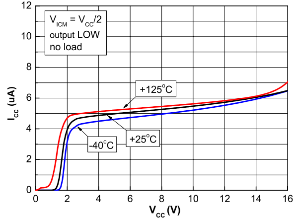
Figure 4. Current consumption vs. supply voltage, output low
