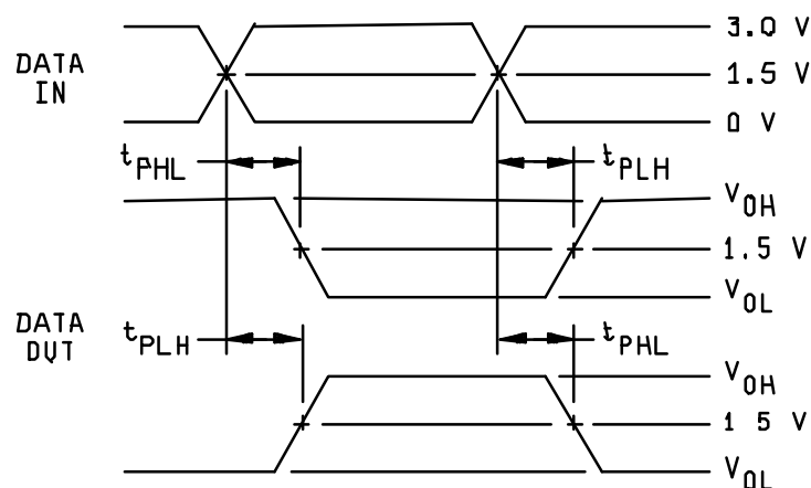
PROPAGATION DELAY TIME
