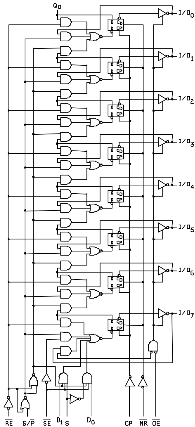
FIGURE 3. Logic diagram.
