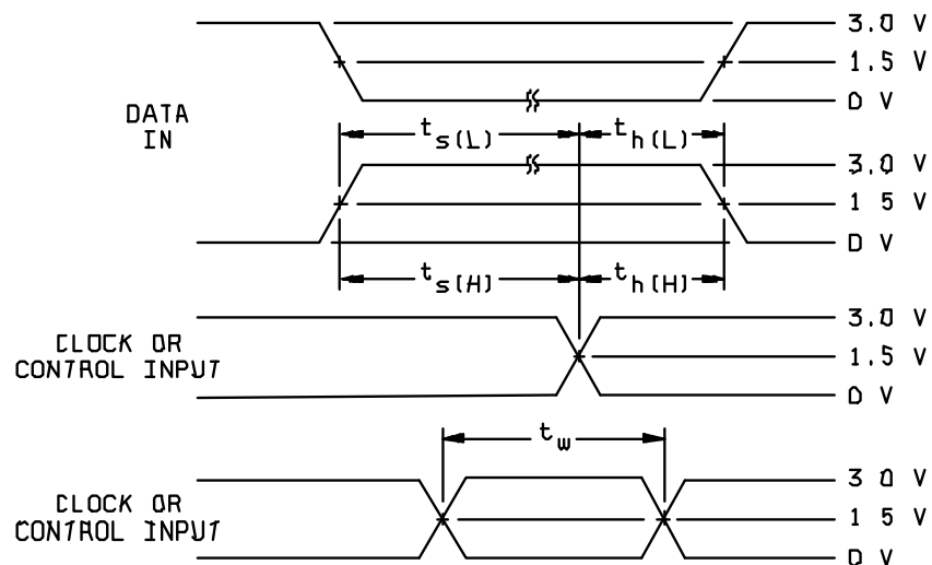
SETUP TIME, HOLD TIME AND PULSE WIDTHS
