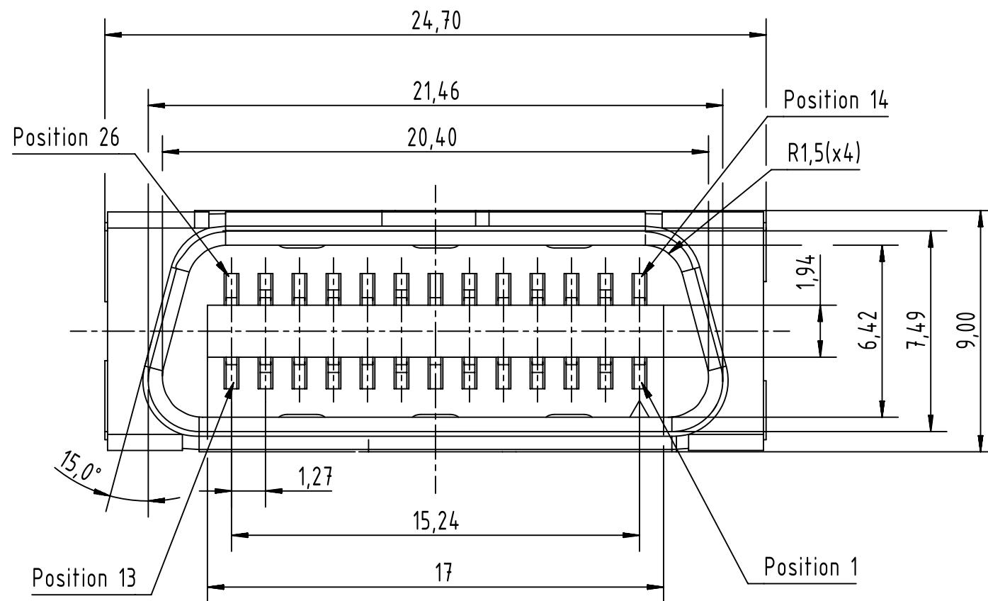
26-pole Cover One With Small Slits
