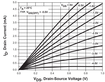
Output Characteristics
