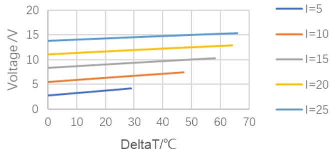
Performance Curves at T_h=27^\circ\text{C}
